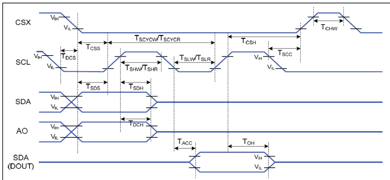
Figure 1 4-wire serial Interface Timing Characteristics
