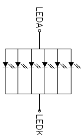
BACKLIGHT CIRCUIT DIAGRAM
